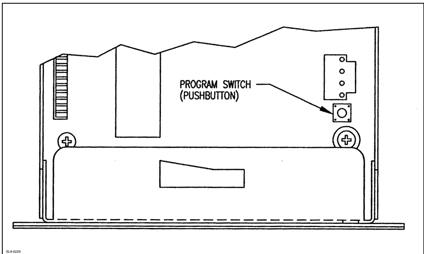
FIGURE 4 - Top View Of Controller.
